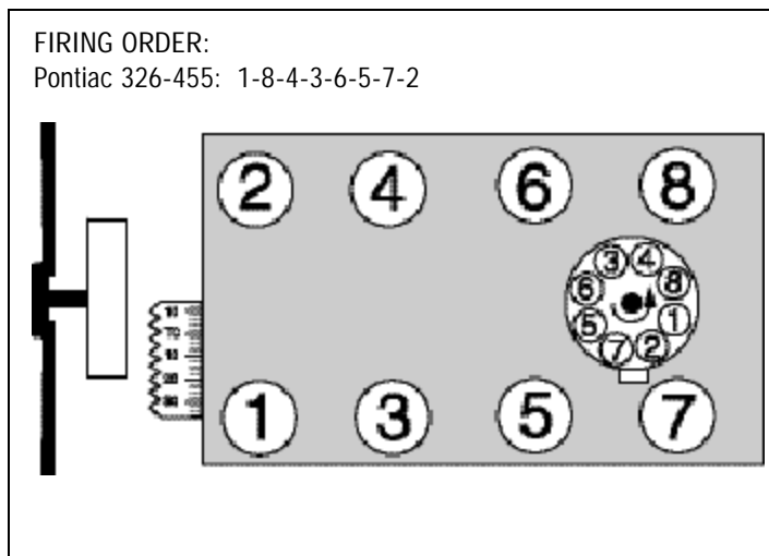
Figure 2 - Firing Order
