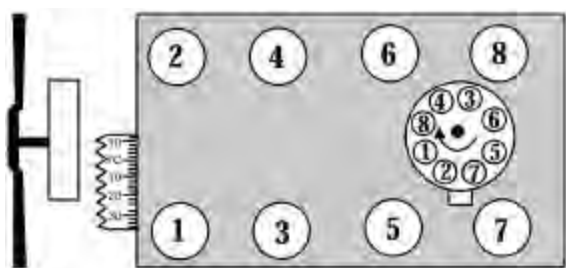
Figure 1 - 350-400 c.i.d Chevrolet V8 Firing Order and Timing Marks
