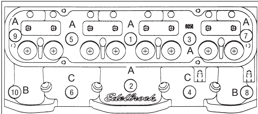
Figure 1- Head Bolt Boss locations and Tightening Sequence
