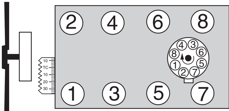
Figure 1- Chevrolet 265-400 c.i.d. V8
