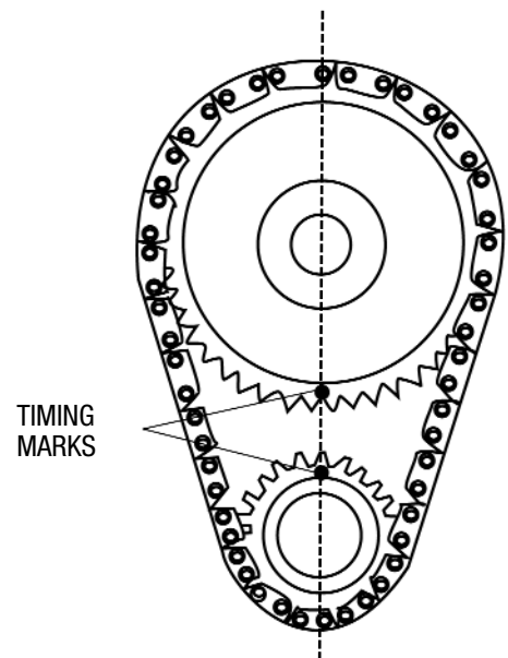
Figure 2- Timing Chain Sprocket Alignment
