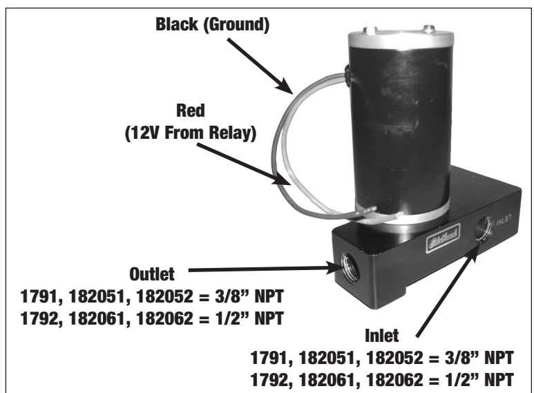
Figure 2 - Fuel Pump
