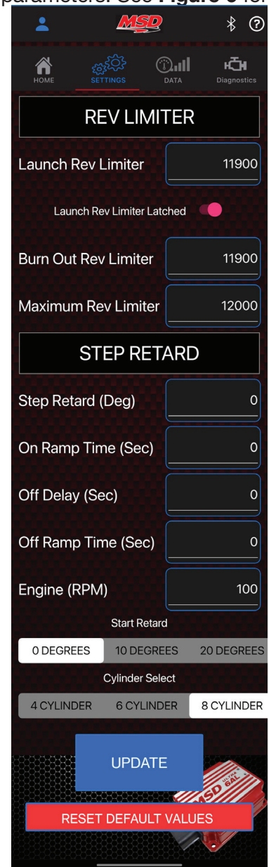
Figure 6. Settings Screen
